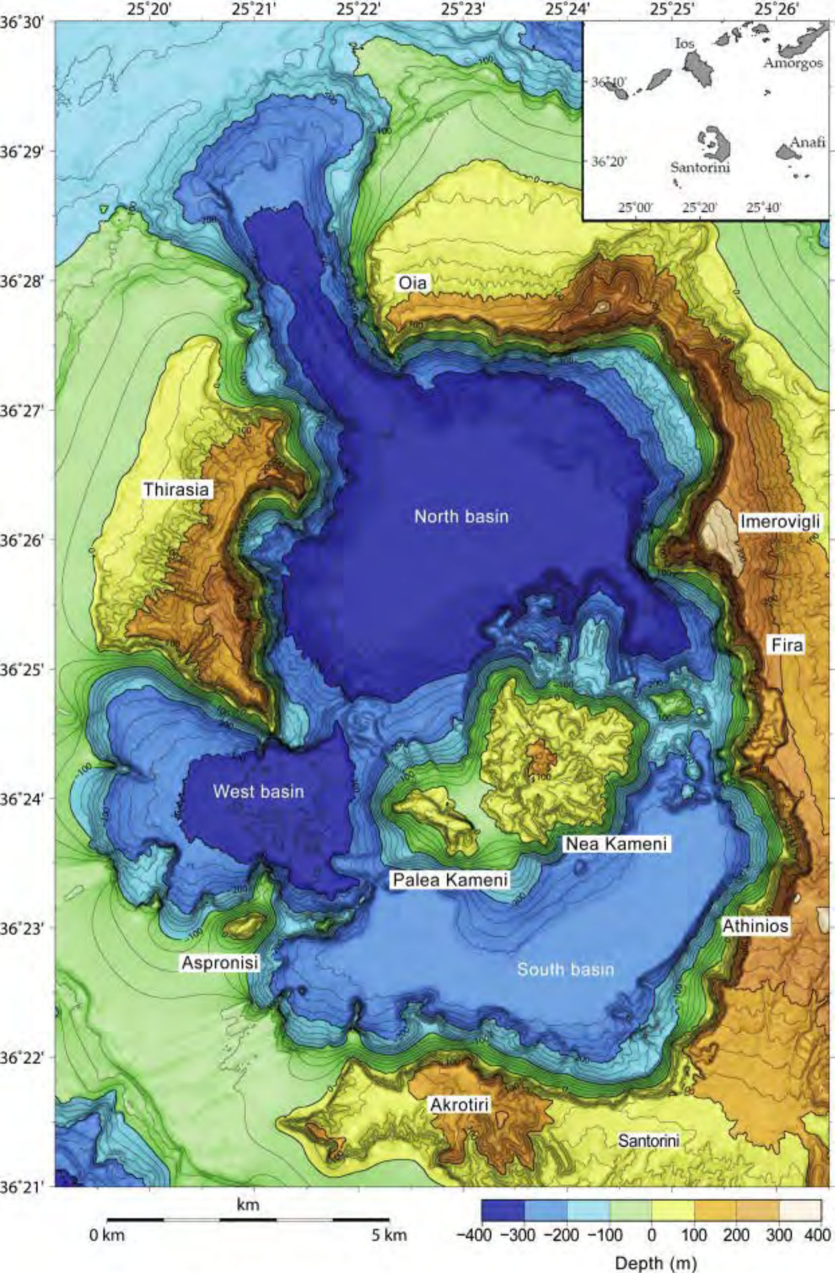
Combined bathymetric and topographic map of Santorini Caldera with 15-m grid resolution - P. Nomikou et al
