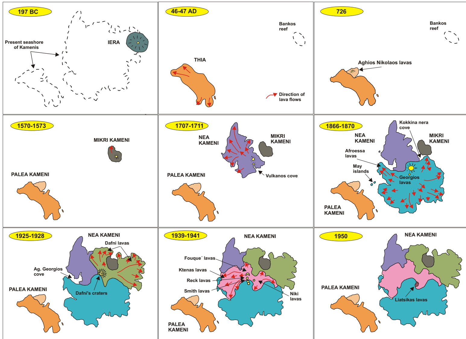
THE CREATION OF PALEA AND NEA KAMENI
